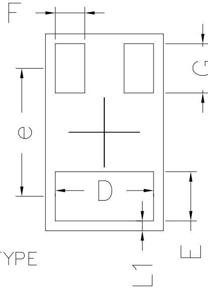
BOTTEM VIEW
